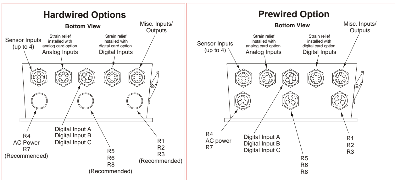
Figure 2: Conduit/Wiring Configuration
