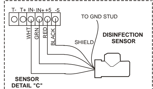
Figure 5: Wiring Diagram for Sensor Inputs and Digital Inputs A-F
